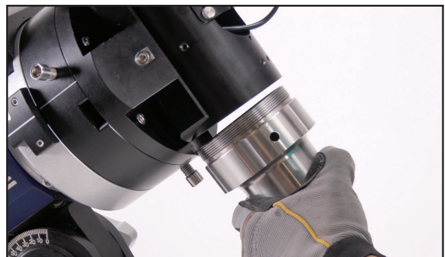
Fig 12: Attach Counterweight Shaft.
