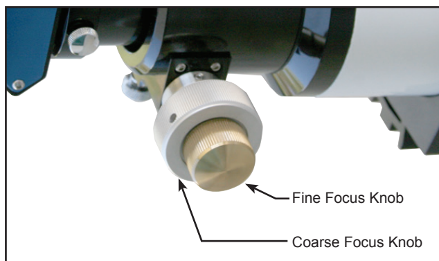
Fig 33: APO Crayford focuser
