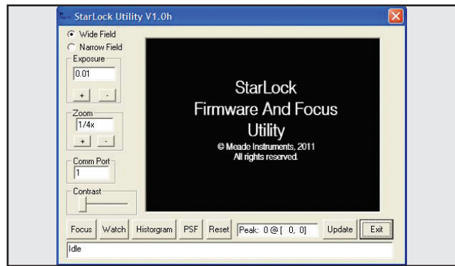
Fig 39: Start-up Screen
